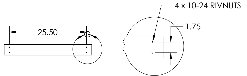
DETAIL G
