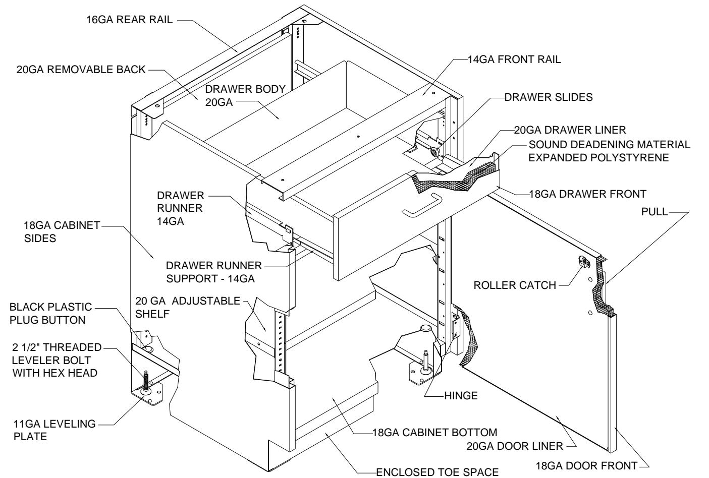
TYP. BASE CABINET
