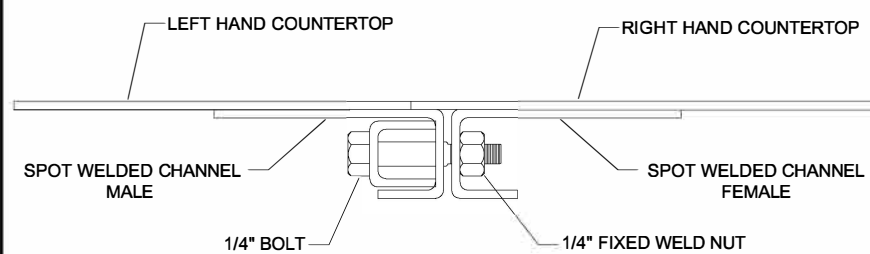
TYPICAL MECHANICAL JOINT DETAIL
