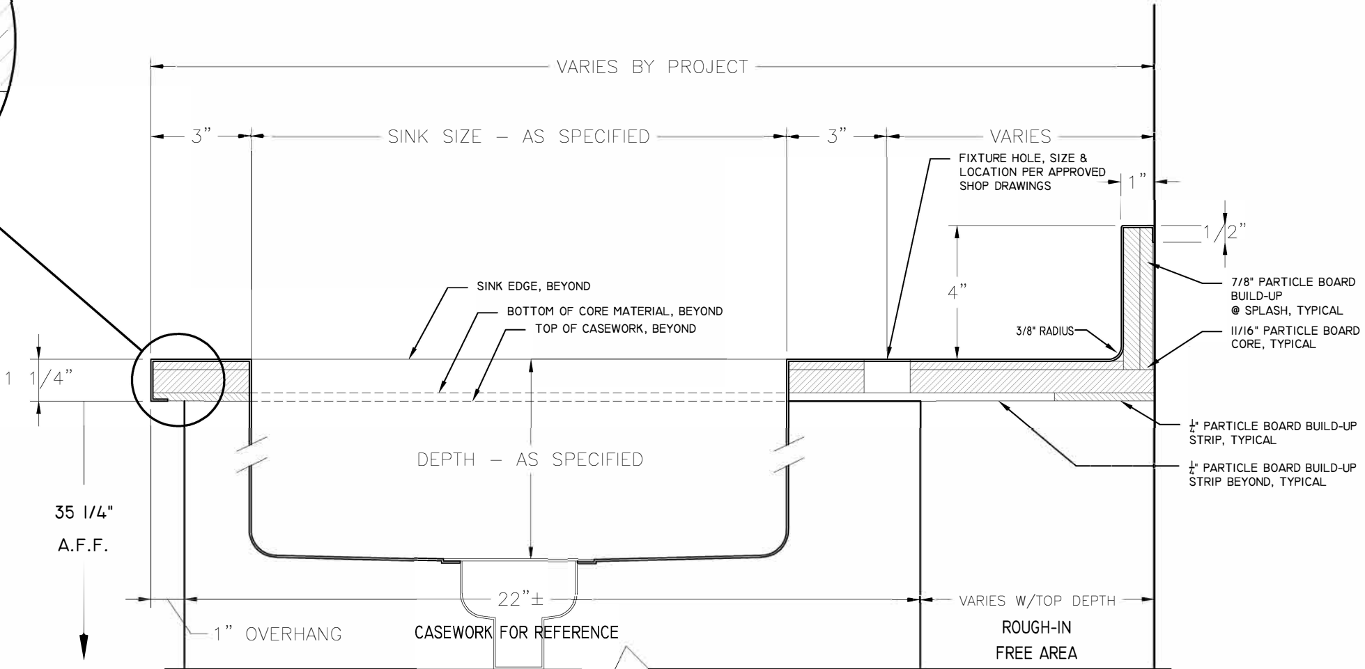
TYPICAL PERIMETER STAINLESS STEEL COUNTER TOP WITH PARTICLE BOARD CORE AND SINK
