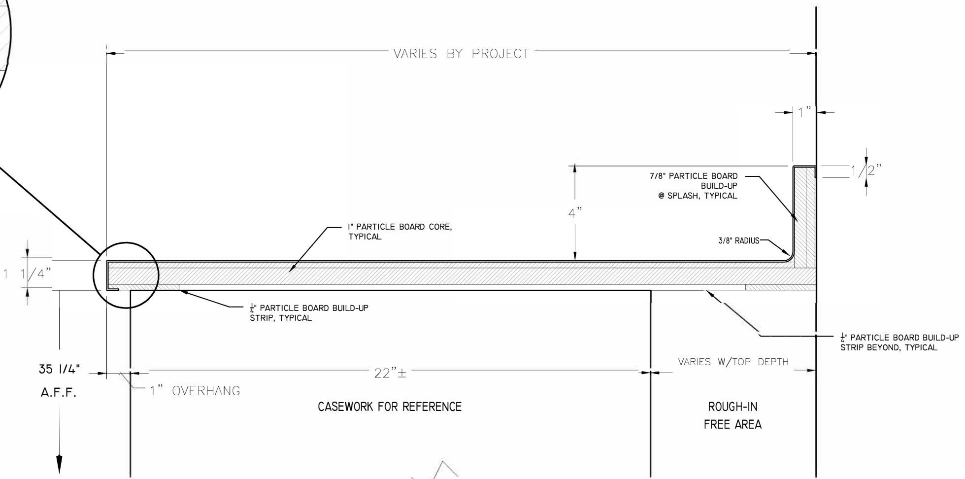
1 TYPICAL PERIMETER STAINLESS STEEL COUNTER TOP WITH PARTICLE BOARD CORE
