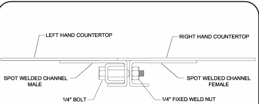
TYPICAL MECHANICAL JOINT DETAIL
