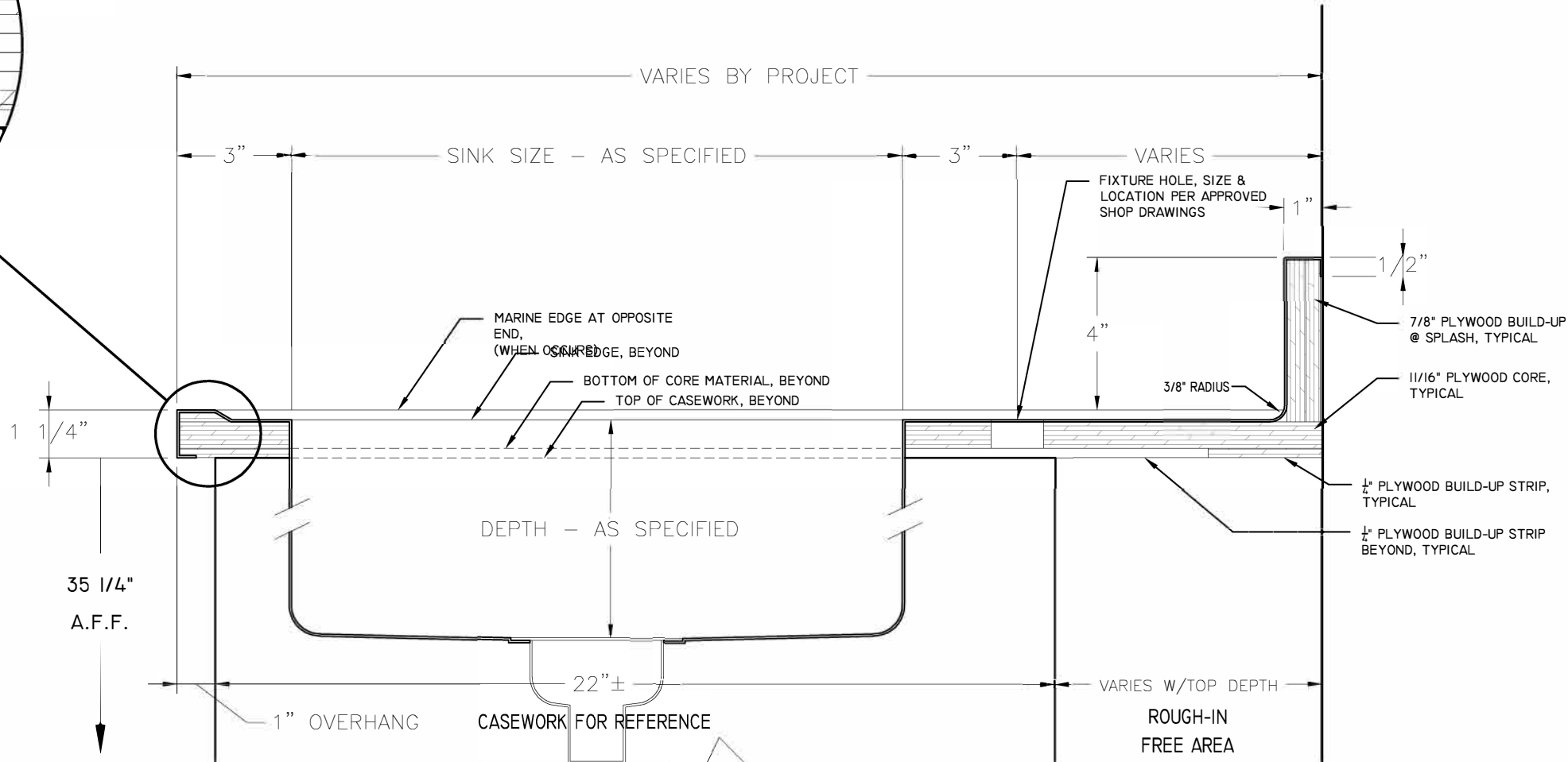
1 TYPICAL PERIMETER STAINLESS STEEL COUNTER TOP WITH MARINE EDGE, PLYWOOD CORE, AND SINK
