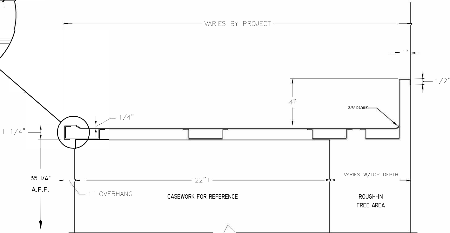
ENLARGED MARINE EDGE DETAIL
