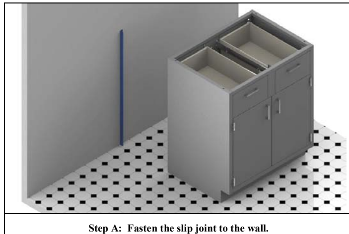
Step A: Fasten the slip joint to the wall.
