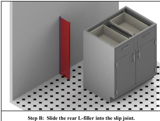
Step B: Slide the rear L-filler into the slip joint.
