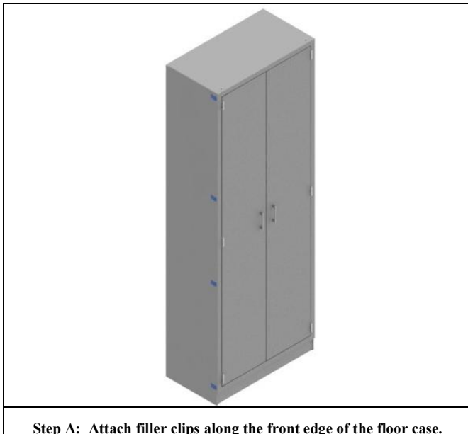
Step A: Attach filler clips along the front edge of the floor case.
