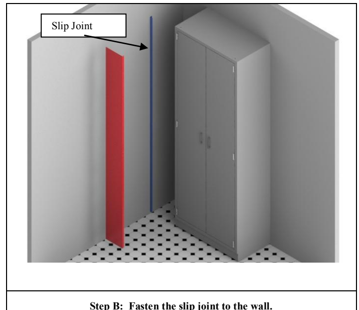
Step B: Fasten the slip joint to the wall.
