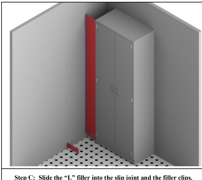
Step C: Slide the "L" filler into the slip joint and the filler clips.
