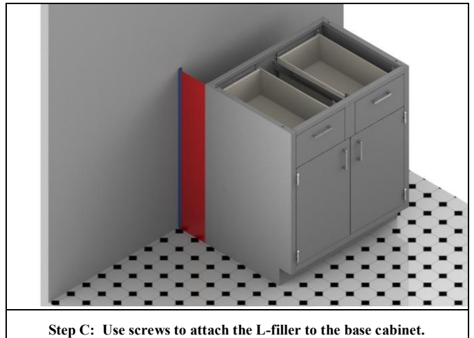
Step C: Use screws to attach the L-filler to the base cabinet.
