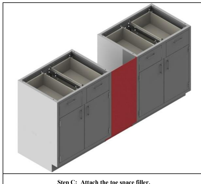
Step C: Attach the toe space filler.
