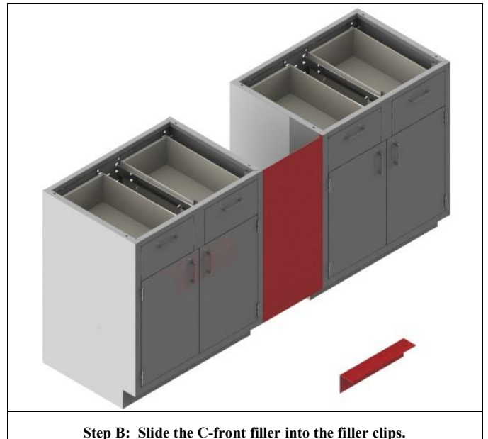
Step B: Slide the C-front filler into the filler clips.
